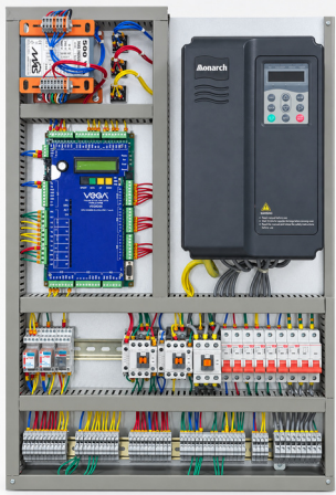
VEGA 200 / MONARCH
